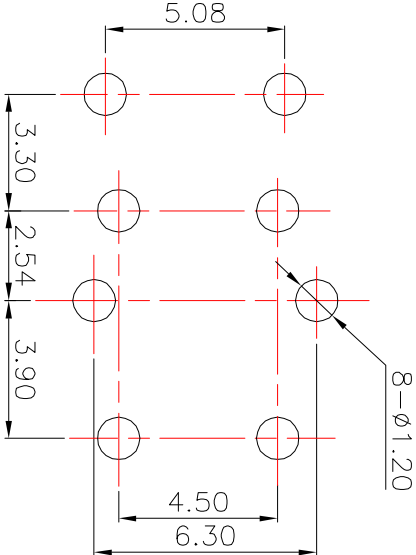
PCBLayout(Pattern Side)
