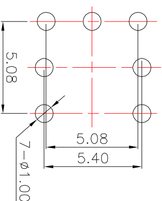
PCBLayout(Pattern Side)
