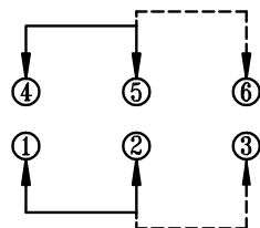
SCHEMATIC (NON-SHORTING)
