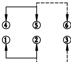
SCHEMATIC (NON-SHORTING)
