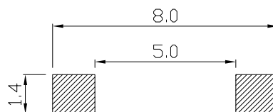
P.C.B MOUNTING PATTERN DIMENSION
