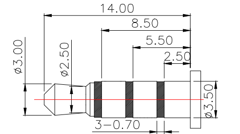
(ø3.50mm 4 POLE PLUG )
