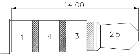
Φ3.5 MATE PLUG
